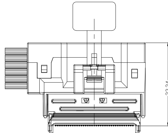
MATING VIEW
