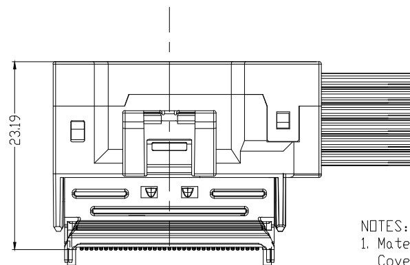
MATING VIEW
