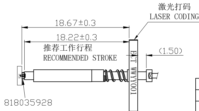
工作状态 WORKING CONDITION
