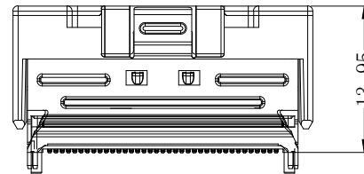
MATING VIEW
