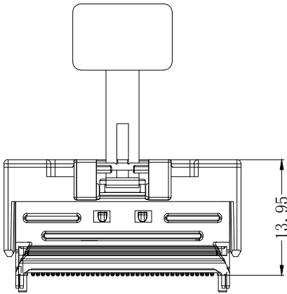
MATING VIEW
